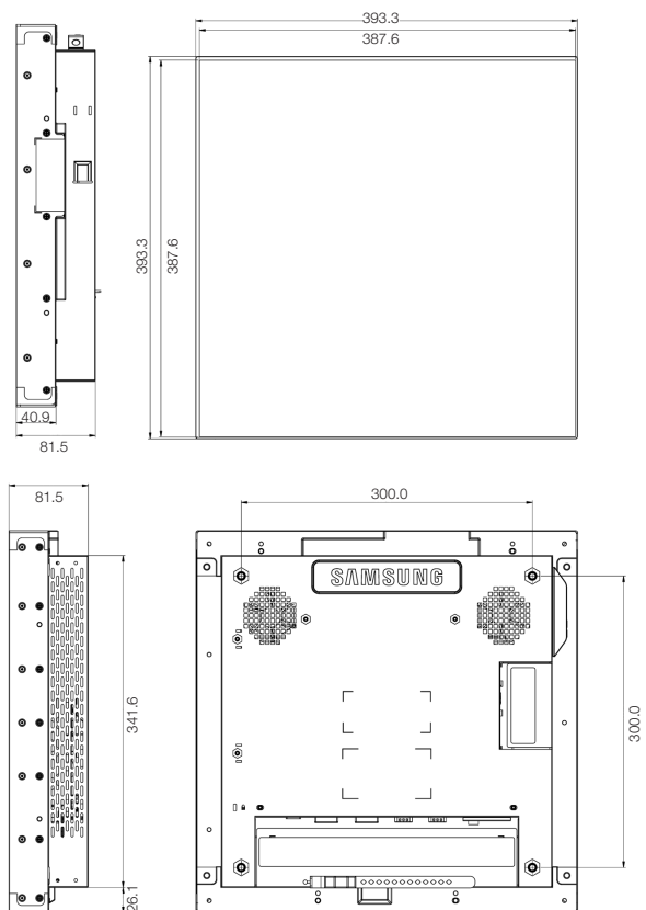
Figure 1. Samsung UD22B schematic
